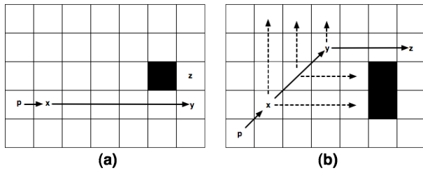
Figure 2: (a) A straight jump from x to y ; the recursion stops due to node z which is forced. (b) A diagonal jump from x to y ; the recursion stops due to a non-failed straight jump. Continuing would mean missing a potential turn due to z .
