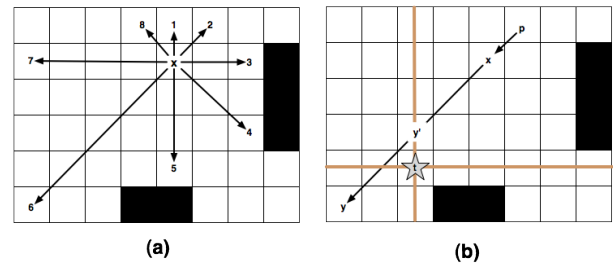
Figure 3: (a) A jump point is computed in place of each grid neighbour of node x . (b) When jumping from x to y we may cross the row or column of the target t (here, both). To avoid jumping over t we insert an intermediate successor y' on the row or column of t (whichever is closest to x ).
