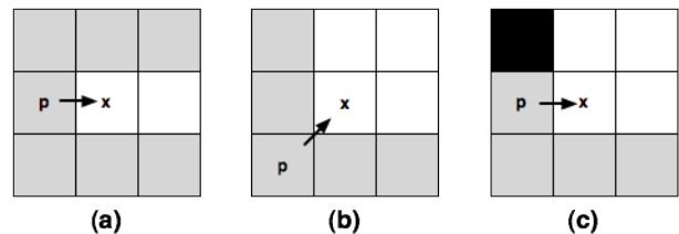
Figure 1: (a) When the move from p to x is straight only one natural neighbour remains. (b) When the move from p to x is diagonal, three natural neighbours remain. (c) Obstacles around x cause some neighbours to become forced.
